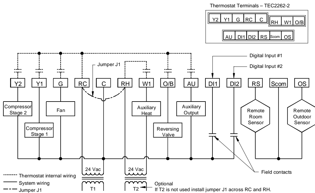
Figure 7: TEC2262-2 Heat Pump Thermostat
