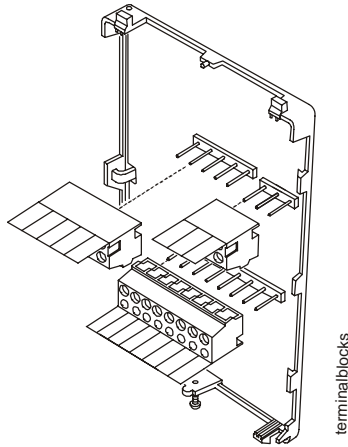
Figure 3: Security Screw
