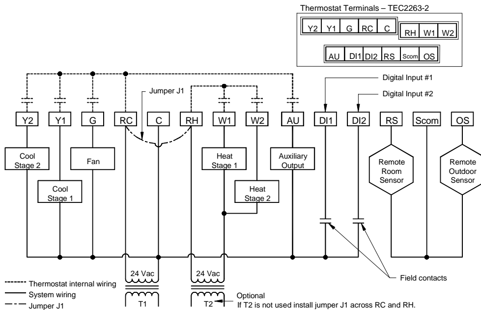
Figure 5: TEC2263-2 Multi-Stage Thermostat
