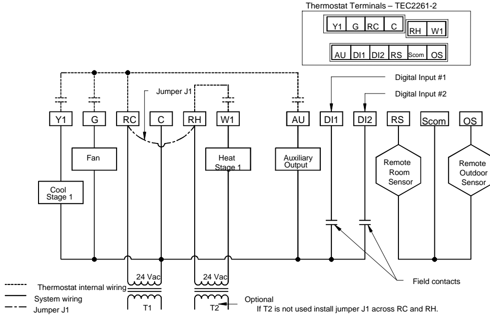
Figure 4: TEC2261-2 Single-Stage Thermostat
