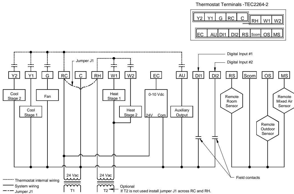
Figure 6: TEC2264-2 Economizer Thermostat
