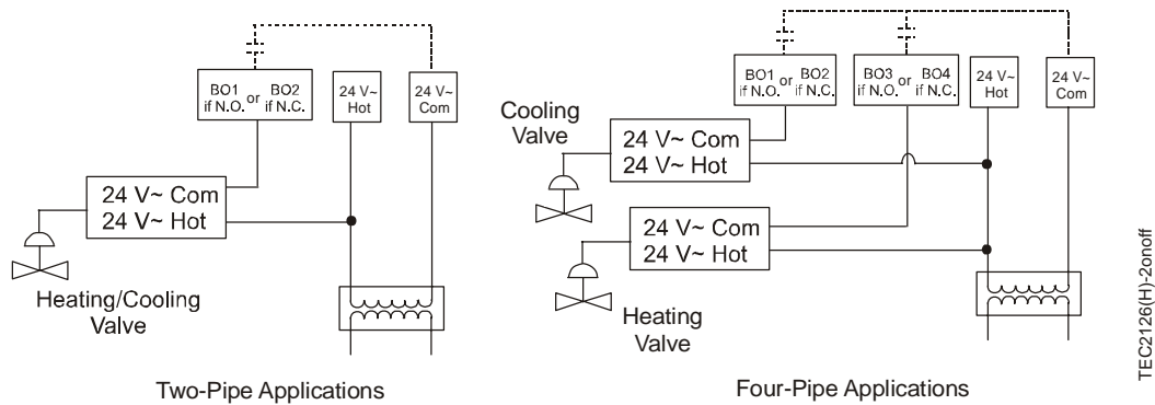
Figure 7: Wiring TEC2126(H)-2 Thermostats for On/Off Control
