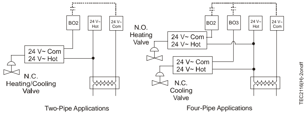
Figure 6: Wiring TEC2116(H)-2 Thermostats for On/Off Control
