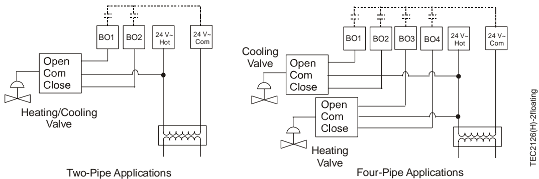
Figure 8: Wiring TEC2126(H)-2 Thermostats for Floating Control
